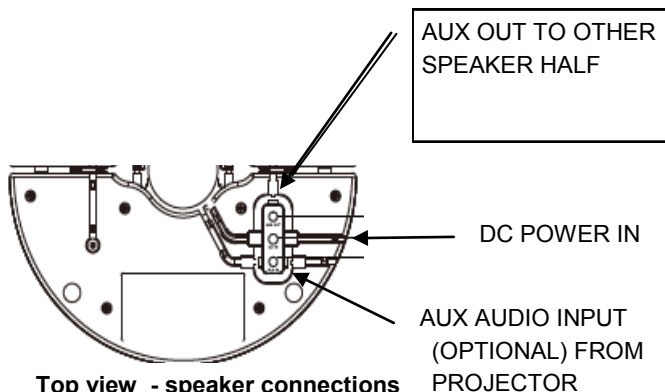
Top view - speaker connections on the powered half .
